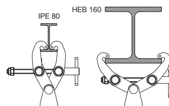
Clamp Range IPE 80 to IPE 160 HEB 80 to HEB 160
